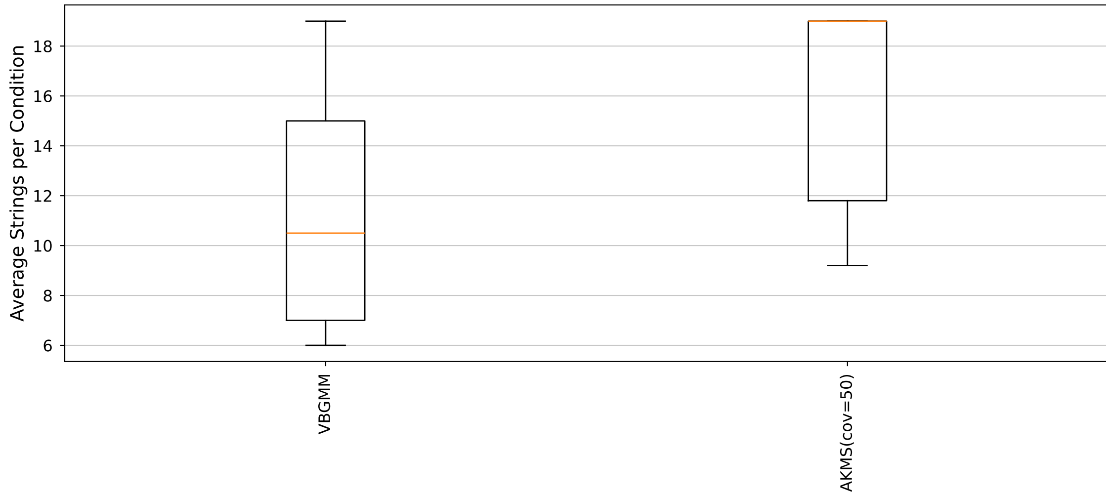
YARA Rules Average Strings per Condition Distribution (Cluster0_Size134 dataset)
